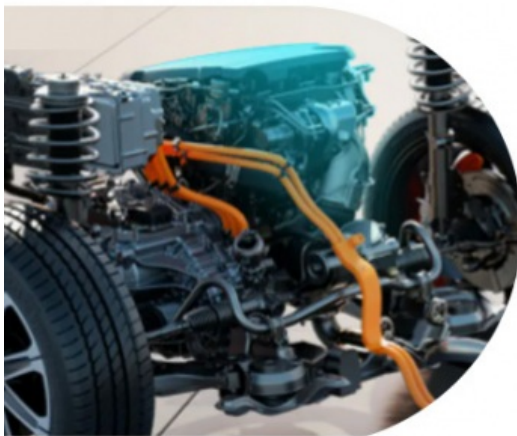
Blue Whale NE15T hybrid dedicated engine, eliminating front-end gear trains and adopting Miller cycle technology to ensure efficiency
